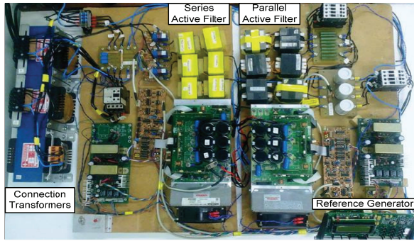
Fig. 15. The dual UPQC prototype.
