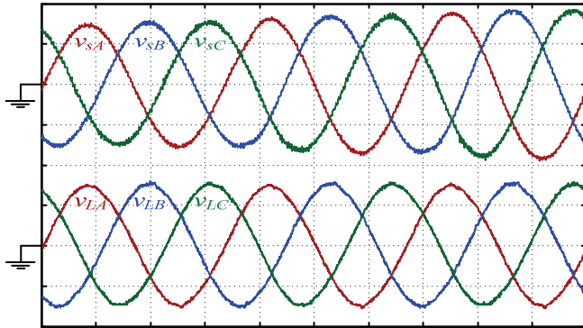
Fig. 20. Source voltages and load voltages (100V/div, 5ms/div) during a voltage swell.
