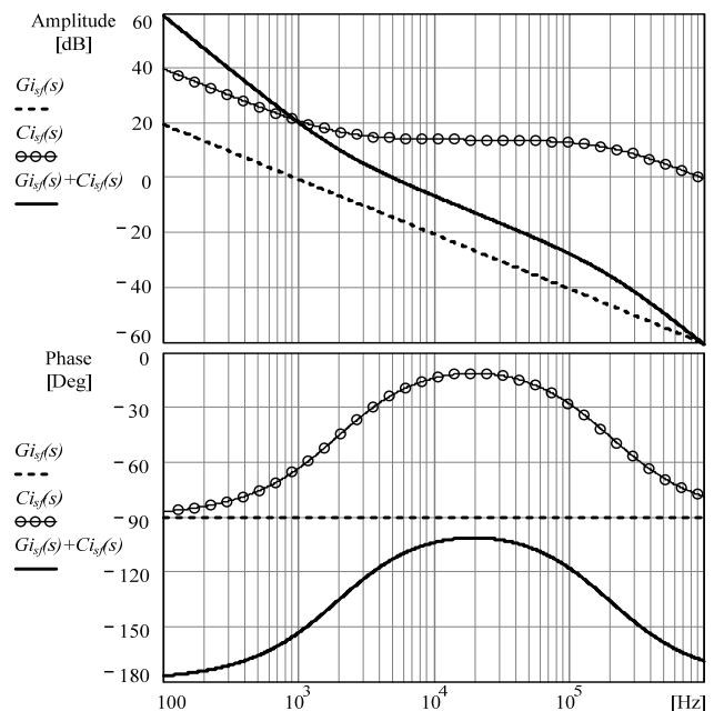
Fig. 5. Current loop frequency response of the series active filter.
