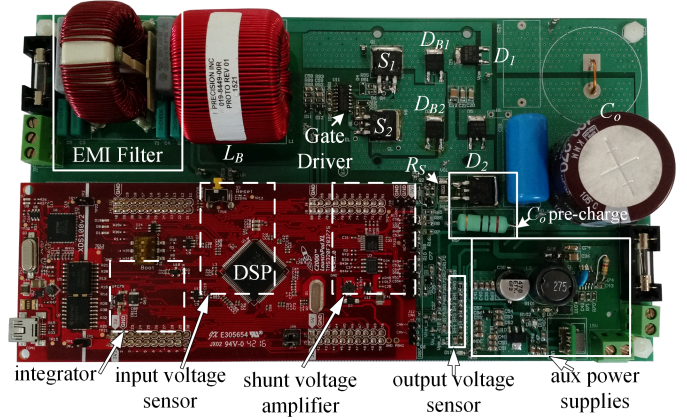
Fig. 12. 300W TPBR prototype using shunt current sensor.
