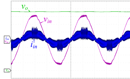
Fig. 14. Instability of LEM-OCC at high emulated resistance. V_{in}^{rms} = 220 V, P_{in} = 58.4 W.
