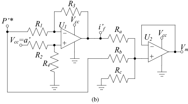
Fig. 10. LEM-OCC-SDS. (a) Block diagram. (b) Analog implementation circuit.
