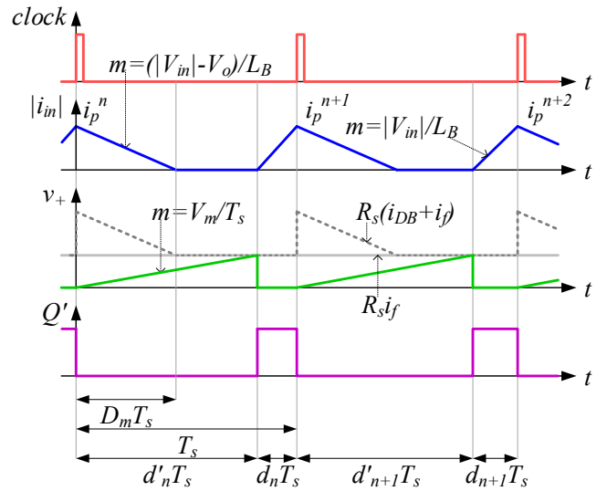
Fig. 8. Waveforms of LEM-OCC with fictitious current during DCM operation.
