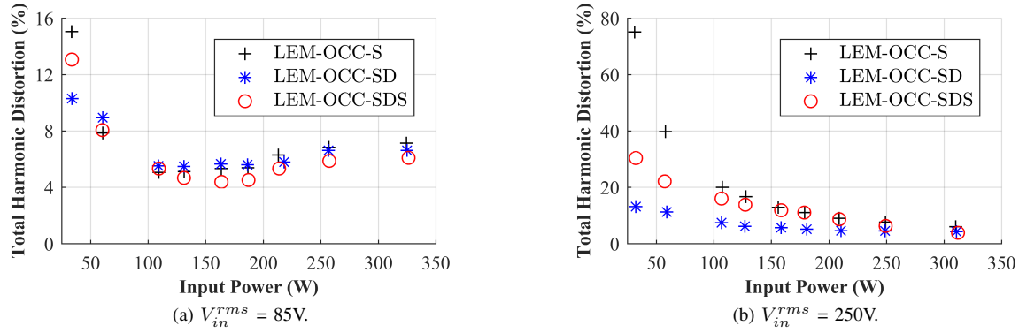
Fig. 20. Experimental results of input current THD.
