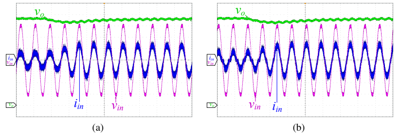
Fig. 18. Experimental results of load step with P_{in}=110W \rightarrow P_{in}=210W . V_{in}^{rms} = 220V . Time: 4ms/div, v_o : 50V/div, v_{in} : 100V/div, i_{in} : 1A/div. (a) LEM-OCC-SD. \Delta V_o = -15V . (b) LEM-OCC-SDS. \Delta V_o = -17V .
