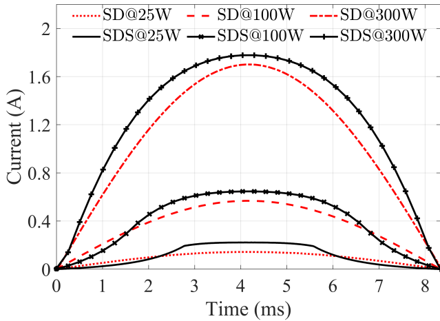
Fig. 11. Average input current of LEM-OCC-SD and LEM-OCC-SDS for different values of P^* . V_{in}^{rms} = 250V . R_f = 361\Omega for LEM-OCC-SD. a = 0.978 and b = 0.0028 for LEM-OCC-SDS.
