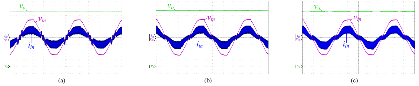
Fig. 15. Experimental results: 25W@85V. Time: 4ms/div, v_o : 50V/div, v_{in} : 50V/div, i_{in} : 500mA/div. (a) LEM-OCC-S. (b) LEM-OCC-SD. (c) LEM-OCC-SDS.
